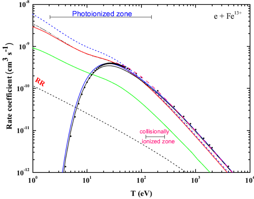
Figure 2 Maxwellian-averaged DR and RR rate coefficients for \text{Fe}^{13+} : blue dashed curve, Maxwellian-average DR rate coefficient for the experimental measurements of Schmidt et al. [7]; black dotted curve, DR calculations of Badnell [13]; red solid curve, our DR rate coefficient in IC-coupling; pink dashed curve, DR data of Jacobs et al. [10]; black circles, DR data fitting of Shull and Steenberg [9]; black solid curve, DR data from the empirical formula of Mewe et al. [8]; blue solid curve, recommended DR data by Mazzotta et al. [11]; green solid curve, total rate coefficient (RR + DR) using R -matrix by Nahar [12]; and gray dashed curve, my RR data. The collisionally ionized zone is as recommended by Bryans et al. [14]. The photoionized zone is taken from Ref. [15].
