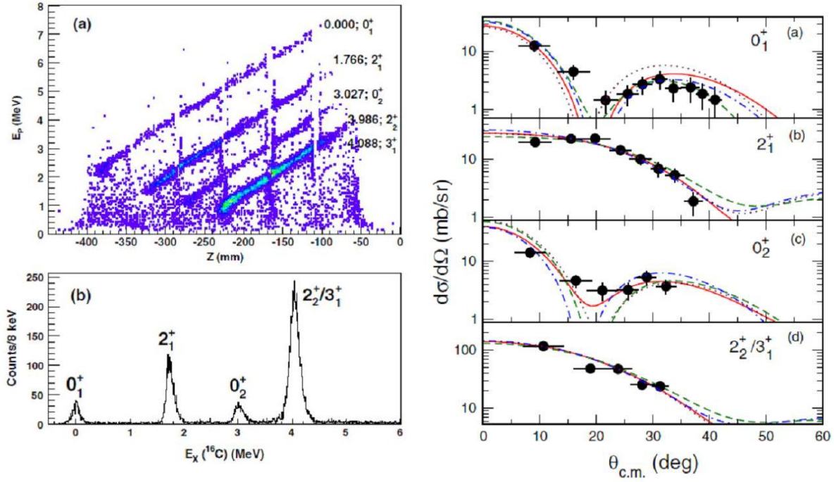
Figure 1: Left: Proton energy-position correlation plot (top) and excitation-energy spectrum (bottom) from ^{15}\text{C}(d,p)^{16}\text{C} reaction. Right: Angular distributions for positive-parity states in ^{16}\text{C} . The curves are distorted-wave Born-approximation calculations using different sets of optical-model parameters.
