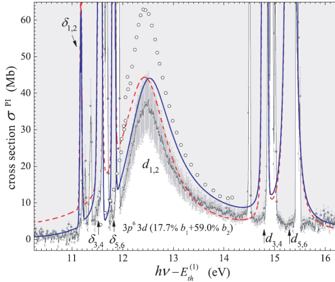
Figure 2 Comparison between computed and experimental PI cross sections for \text{Sc}^{2+} . Red dashed curve: present theoretical PI cross sections in lowest order, convolved with the experimental energy spread of 44 meV. Blue solid curve: higher-order MCBP results including resonance-continuum interference effects. Open circles: segment of the PI cross section computed by Sossah et al. [6] in the vicinity of the d_{1,2} resonances; (black points with dark gray error bars) high-resolution merged photon-ion beams experimental data of Schippers et al. [5]. The background areas below and above the experimental data are shaded as white and light gray, respectively, to show more clearly the high narrow experimental resonances in the 11- to 12-eV and 14.5- to 15.5-eV regions. The energy scale is given relative to the first ionization threshold E_{\text{th}}^{(1)} = 24.75684 eV.
