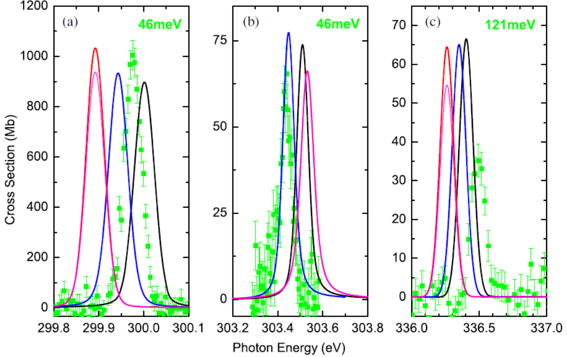
Figure 2 Present R -matrix cross section vs. experimental and earlier R -matrix results [2] for the 1s \rightarrow 2p and 3p resonances of C^{3+} : Green curve represents the experimental data. Black and blue curves show previous R -matrix results in IC- and LS -coupling schemes, respectively. Red and magenta curves show the present R -matrix photoabsorption and photoionization results, respectively. All theoretical cross sections are convolved with an FWHM Gaussian given by the experimental resolution; the 1s[2s2p(^3P)]^2P and 1s[2s2p(^1P)]^2P resonances are measured with a spectral resolution of 46 meV whereas the 1s[2s3p(^3P)]^2P resonance is measured with a resolution of 121 meV.
