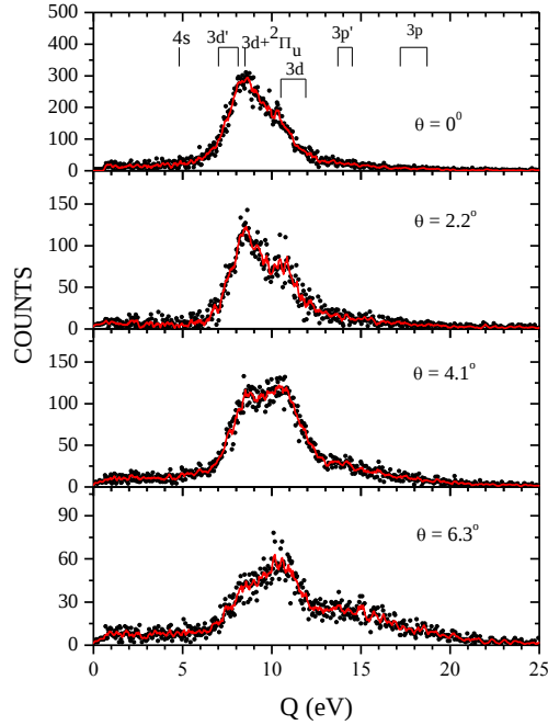
Figure 1. Translational energy-gain spectra for single-electron capture by 100 eV \text{Ne}^{4+} ions from \text{CO}_2 at different projectile laboratory scattering angles.
