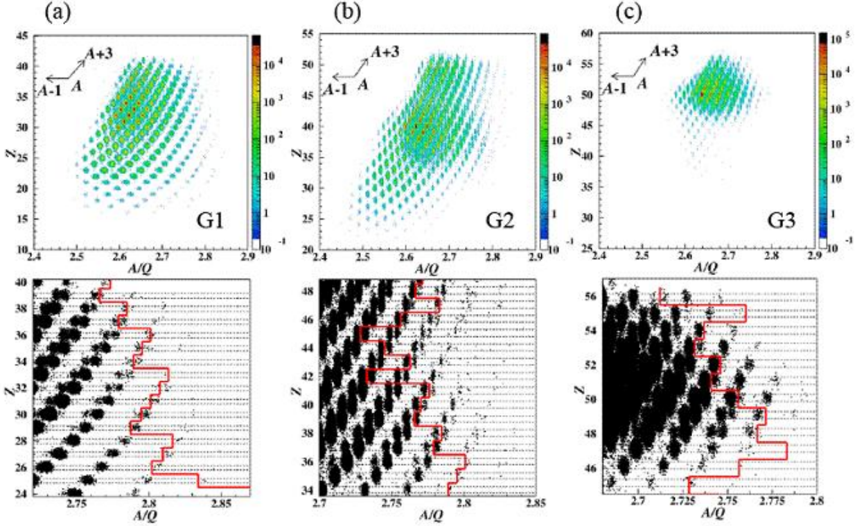
Figure 2 - Z versus A/Q plots for the fission fragments produced in the ^{238}\text{U}+\text{Be} reaction (a and b) and the ^{238}\text{U}+\text{Pb} reaction (c) at 345 MeV/nucleon. Each column represents a different spectrometer optics setting. The arrows in the upper panels indicate that the isotopes located on the upper right hand and on the left hand correspond to those with mass numbers A+3 and A-1, respectively. The lower panels show the PID plot enlarged around the regions of new isotopes, where the red lines indicate the known frontier and the dotted horizontal lines show the Z gates.
