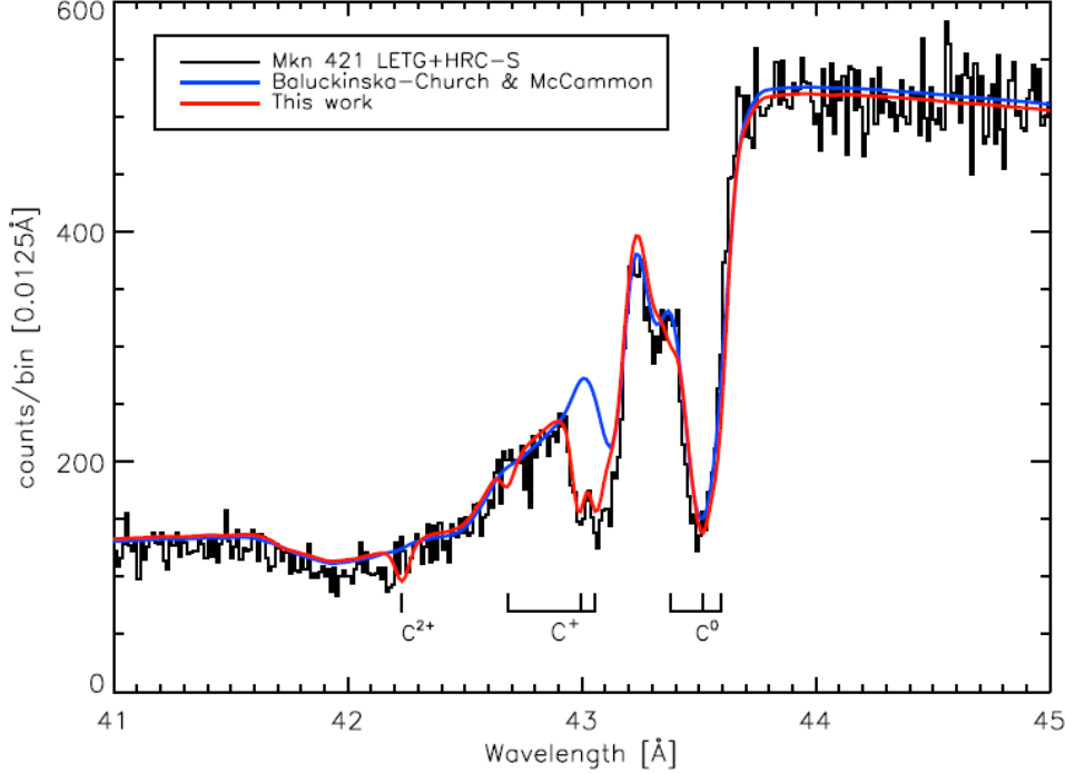
Figure 3 Carbon K-edge region of the X-ray spectrum of the bright blazar Mkn 421 observed by the Chandra LETG+HRC-S. The edge absorption is predominantly due to the polyimide UV-optical/ion blocking filter on the HRC-S instrument, although ISM absorption contributions are also present. Two fits to a power-law continuum model with photon index \Gamma = 2.0 , absorbed by an intervening ISM corresponding to a neutral H column density of 1.5 \times 10^{20} \text{ cm}^{-2} , are shown. These differ significantly only in the carbon cross sections employed: the neutral C cross section of Ref [3]; and C, \text{C}^+ , and \text{C}^{2+} cross sections reported here. In the latter case, the C ion fractions were 20% C, 60% \text{C}^+ , and 20% \text{C}^{2+} . The effect of the \text{C}^+ resonances is clearly visible in the vicinity of 43 Å.
