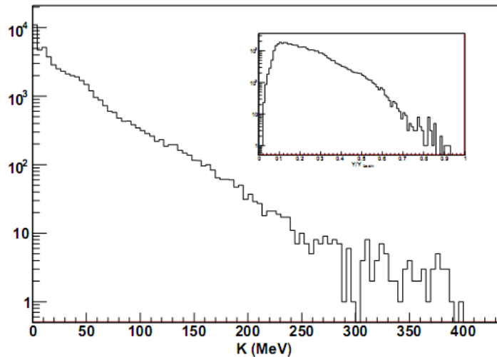
Figure 2 - Neutron energy spectra from the ^{48}\text{Ca}+^{124}\text{Sn} reaction in NSCL experiment #05049. Note that the neutron energies well above 200 MeV are achievable, meaning that high particle rapidity should be observed. The inset shows the rapidity distribution of the produced neutrons in the lab frame (relative to the beam), indicating production at relative rapidities above 0.7 where the sensitivity to the effective masses is greatest. Only a fraction of the data is shown.
