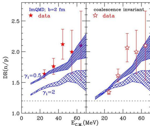
Figure 3 - The free neutron-proton double-ratio (left panel), and the coalescence- invariant neutron-proton double-ratios (right panel) plotted as a function of kinetic energy of the nucleons. The shaded regions represent calculated results from the ImQMD simulations at b = 2 fm. Experimental data is shown. 3
