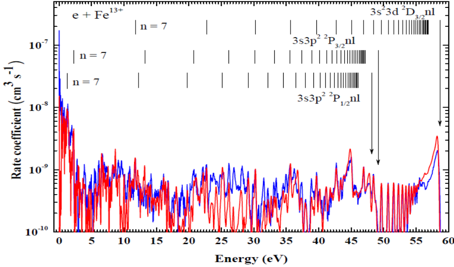
Figure 1 Comparison of the DR rate coefficients with the TSR measured merged-beams electron-ion recombination rate coefficient for \text{Fe}^{13+} from intra-shell \Delta n_c = 0 transitions: blue solid curve, experimental measurements by Schmidt et al. [7]; red solid curve, our MCBP results. The expected DR resonance positions are represented by vertical bars using the hydrogenic Rydberg formula.
