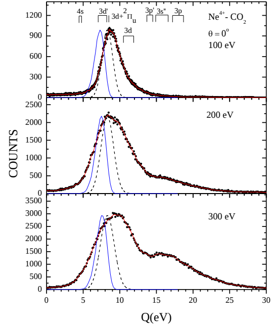
Figure 2. Translational energy-gain spectra for single-electron capture by \text{Ne}^{4+} ions \text{CO}_2 at different projectile impact energies and 0^\circ scattering angles.
