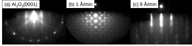
FIG. 1. The reflection high energy electron diffraction (RHEED) patterns collected from (a) a clean \text{Al}_2\text{O}_3(0001) surface and following \text{CeO}_2 growth on \text{Al}_2\text{O}_3(0001) at \sim 650^\circ\text{C} under \sim 2.0 \times 10^{-5} Torr of \text{O}_2 plasma for the growth rates of (b) 1 \text{\AA}/\text{min} and (c) 9 \text{\AA}/\text{min} , indicating the 3-D island growth and 2-D layer growth, respectively.
