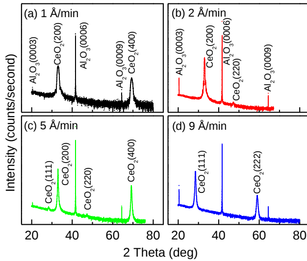
FIG. 2. High-resolution x-ray diffraction (HRXRD) patterns measured from \text{CeO}_2 thin films grown on \text{Al}_2\text{O}_3(0001) for the growth rates of (a) 1 \text{\AA}/\text{min} , (b) 2 \text{\AA}/\text{min} , (c) 5 \text{\AA}/\text{min} and (d) 9 \text{\AA}/\text{min} , indicating the change in orientation with the increase in growth rate.
