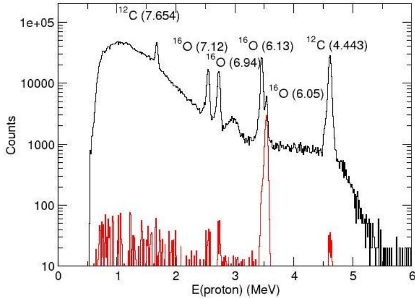
Figure 2. Proton-energy spectra measured in HELIOS from ^{16}\text{O}(p,p')^{16}\text{O}^* inelastic scattering for proton singles (black) and coincidences with e^+e^- (red). The 0^+ excited state of ^{16}\text{O} stands out clearly in the coincidence spectrum. Peaks from a ^{12}\text{C} impurity in the target are also indicated.
