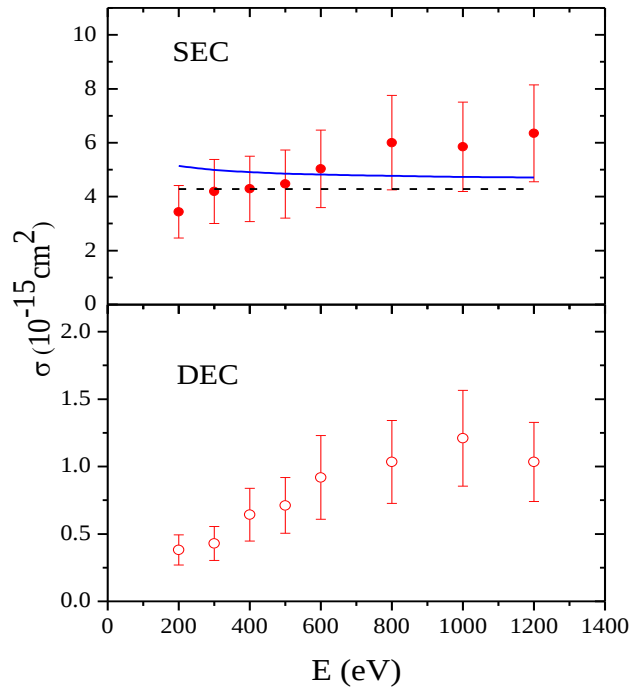
Figure 4. Total cross sections for single-and double-electron capture by \text{Ne}^{4+} ions from \text{CO}_2 . Solid curve, MCLZ calculations; dashed curve, COB model.
