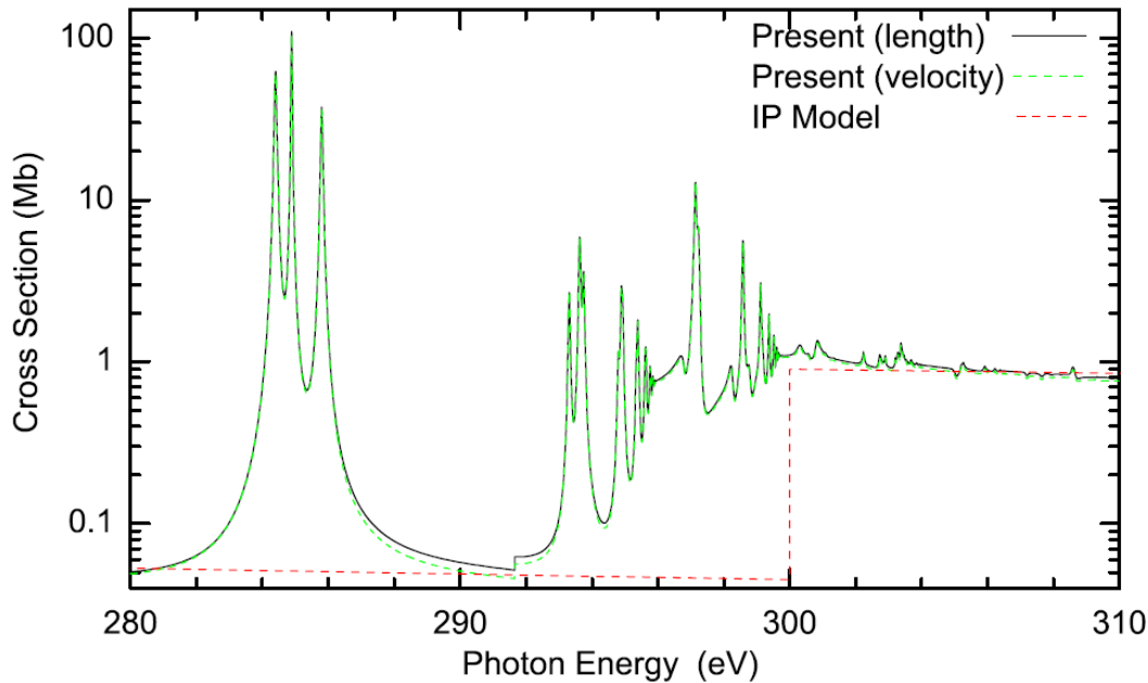
Figure 1 Carbon photoabsorption cross sections: R -matrix length and velocity results compared to the independent-particle results [1].
