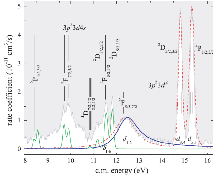
Figure 1 Comparison of the TSR measured \text{Sc}^{3+} PR rate coefficient [4] (white area) with the present lowest-order, perturbative multiconfiguration Breit-Pauli (MCBP) results in the region of the 3p^5 3d 4s (solid green curve) and 3p^5 3d^2 (dashed red curve) resonances. The theoretically designated d_{1,2} resonances required an artificial shift by 0.691 eV to higher c.m. energies in order to align well with the measured spectra. The broad d_{1,2} resonances (solid blue curve) are also described to next-highest order, thereby including dielectronic recombination (DR) and radiative recombination (RR) interference effects.
