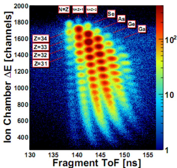
Figure 1 - Particle identification spectrum of the beam-like residues in coincidence with HiRA detected in the S800 focal plane and produced in reactions with the ^{70}\text{Se} secondary beam.
