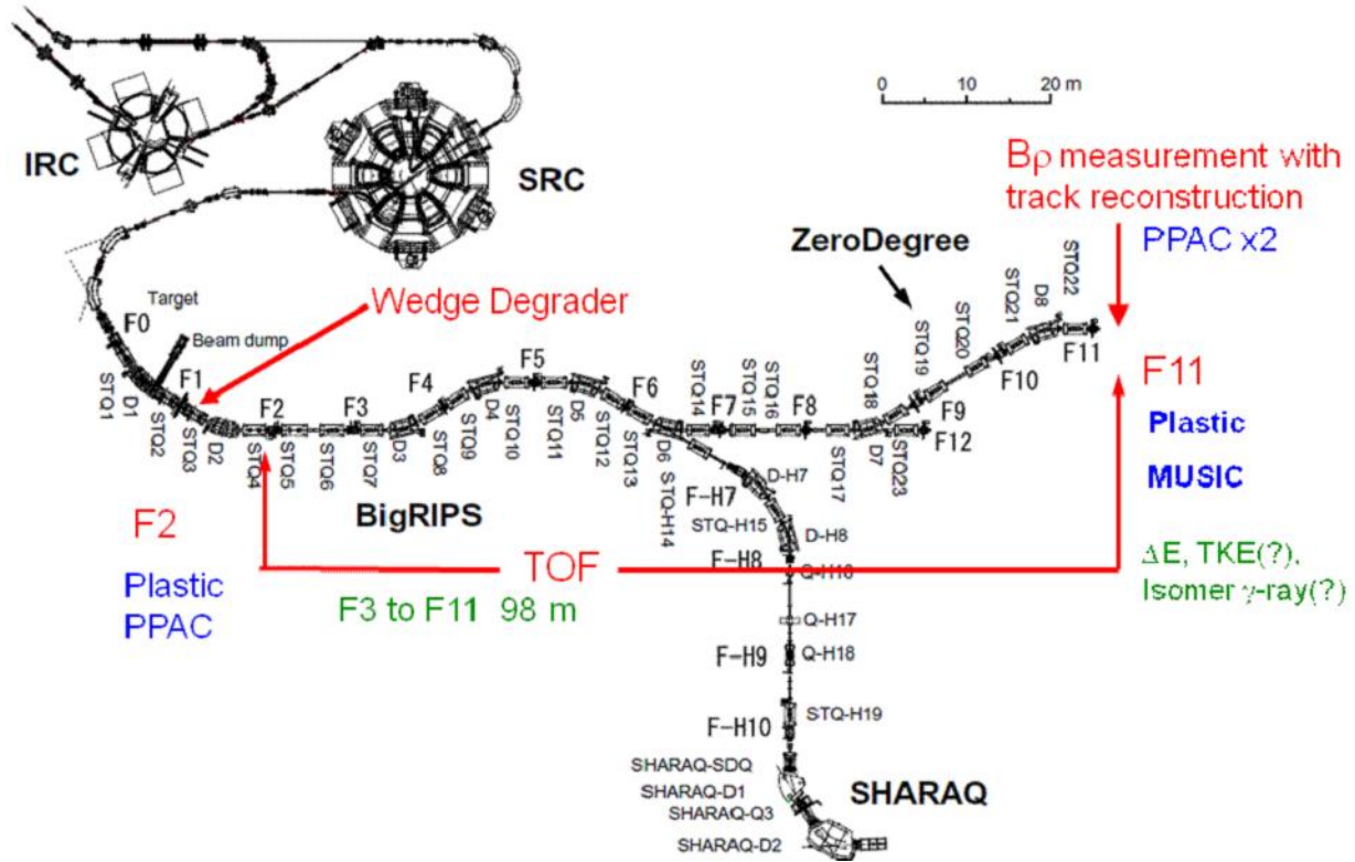
Figure 1 - Schematic diagram of the BigRIPS-Zero Degree Spectrometer device used for the new isotope search experiment and preliminary optics tests for the mass measurement experiment.
